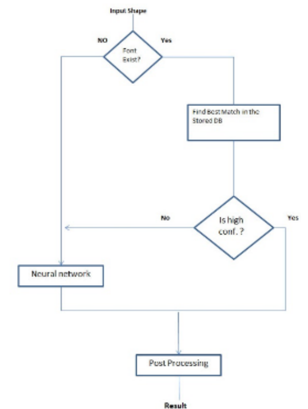
Figure 03 Arabic Text Recognition flow
